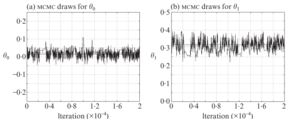
Fig. 1. The first 20 000 Markov chain Monte Carlo draws of (a) \theta_0 and (b) \theta_1 , with the lattice data simulated as in Table 1 at parameter values \theta_0 = 0.0 and \theta_1 = 0.3 . The analytically computed posterior mode appears as an unbroken line, while the simulation average, over 100 000 iterations, is shown as a dashed line.
